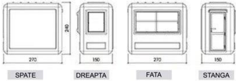
CABINA PAZA 2700X1500X2400 mm
